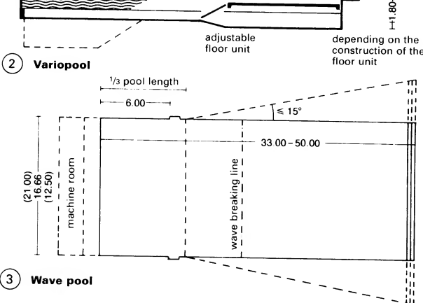
③ Wave pool
